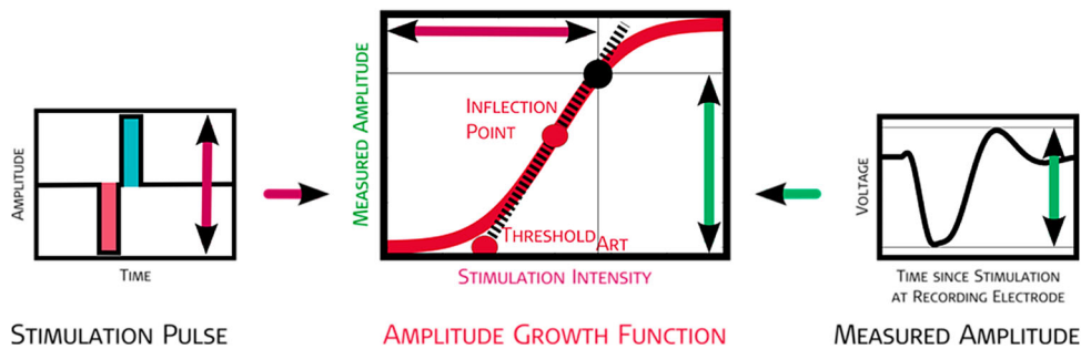
Figure 4 Graphical representation of the AGF and the measurement paradigm fitting function used. The algorithm of the fitting function uses at least four data points. A maximum of two data points were below threshold, i.e. a minimum of two visible ECAPs were used for the determination of AGF threshold and slope. The black point is an example for one amplitude measured in an AGF. The stimulation amplitude (vertical purple arrow) is plotted versus the recorded voltage (vertical green arrow). The inflection point and the threshold are derived from an exponential function fitted to all points measured in an AGF (all derived values are in red).
