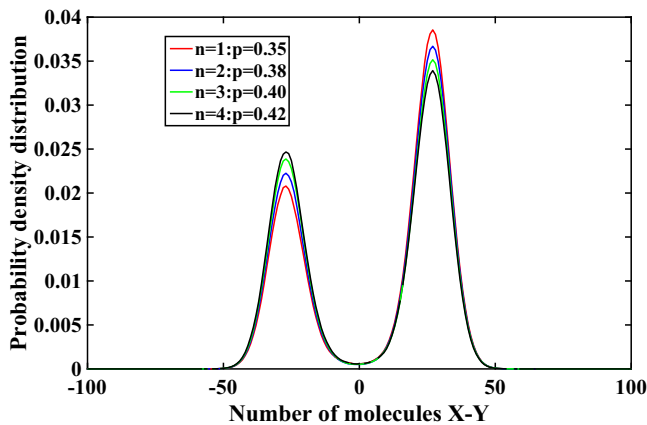
FIG. 5. Equilibrium distribution of toggle-switch circuit for \tau = 2 . p shows the probability of X < Y . Recall that in the DSS, P(X < Y) \sim 0.5 .
