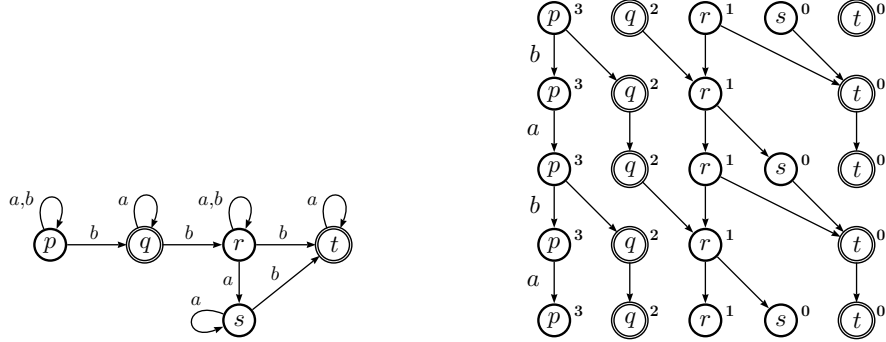
FIGURE 1. Left, the NBW \mathcal{A} , in which all states are initial. Right, the rejecting run DAG G of \mathcal{A} on w = babaabaaba\dots . Nodes are superscripted with the prospective ranks of Section 2.
