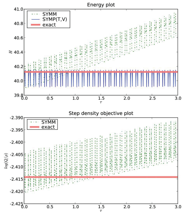
Fig. 4 Results from example 4 (upper). Comparison of energy behaviour for the methods SYMM and SYMP( T, V ) additional first integral \log(Q(z)/Q ) corresponding to step-size density objective for the SYMM method
