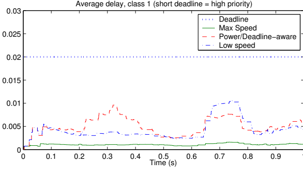
Figure 6.7 Average delay for the high-priority class.
