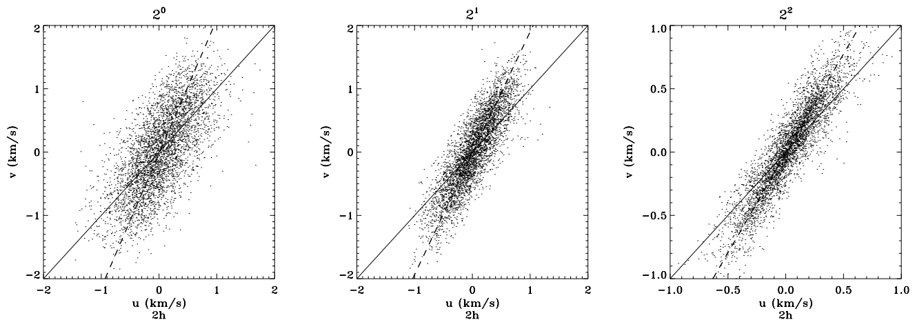
Fig. 4. For three length scales ( 2^0 , 2^1 , 2^2 ), we represent the actual velocity ( v which is either v_x or v_y ) as a function of the measured velocity u for a two-hours average. The clouds represent the 45^2 grid points. The best fits (dashed line) show that granules underestimate actual velocities by a factor which varies from 2.1 at small scales ( 2^0 ) to 1.6 at large scales ( 2^2 ).
