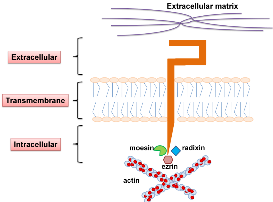
Figure 4. CD44
