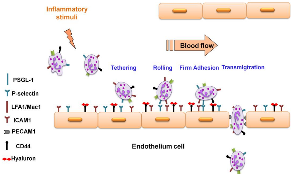
Figure 2. Recruitment process.
