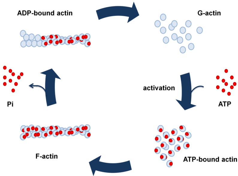
Figure 3. Actin Polymerization
