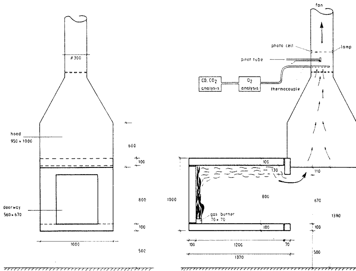
Figure 1 Test configuration for model scale room test. (Dimensions in mm.)
