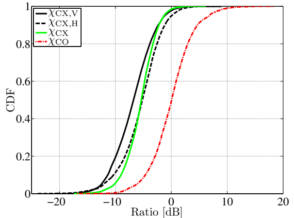
Fig. 2. The CDF of cross- and co-polarization ratios.
