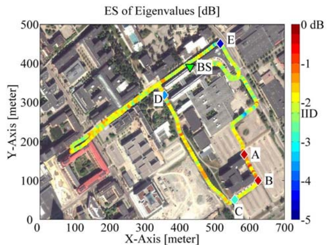
Fig. 1. The ES of channel eigenvalues along the measurement route.
