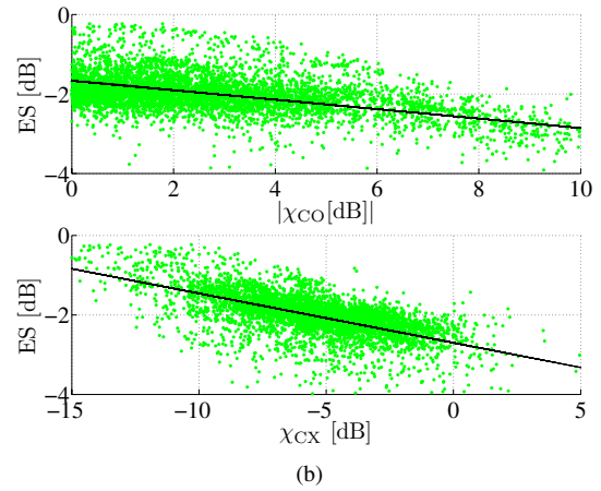
Fig. 5. Dependence between CPR and XPR and their impacts to the ES performance.
