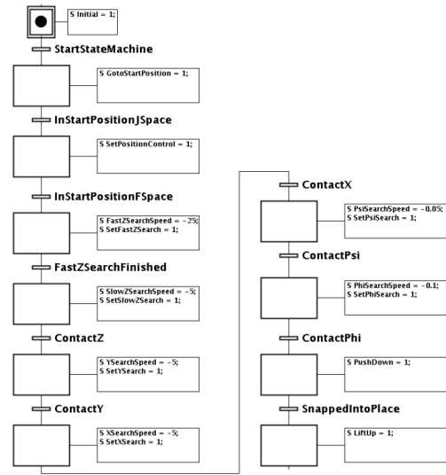
Fig. 7. The SnapFit state machine as an SFC
