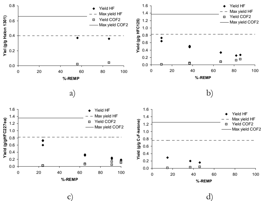
Figure 38. Yields of halogen containing combustion products from the tests with: a) Halon 1301, b) HFC 125, c) HFC 227ea and d) C 6 F-ketone.
