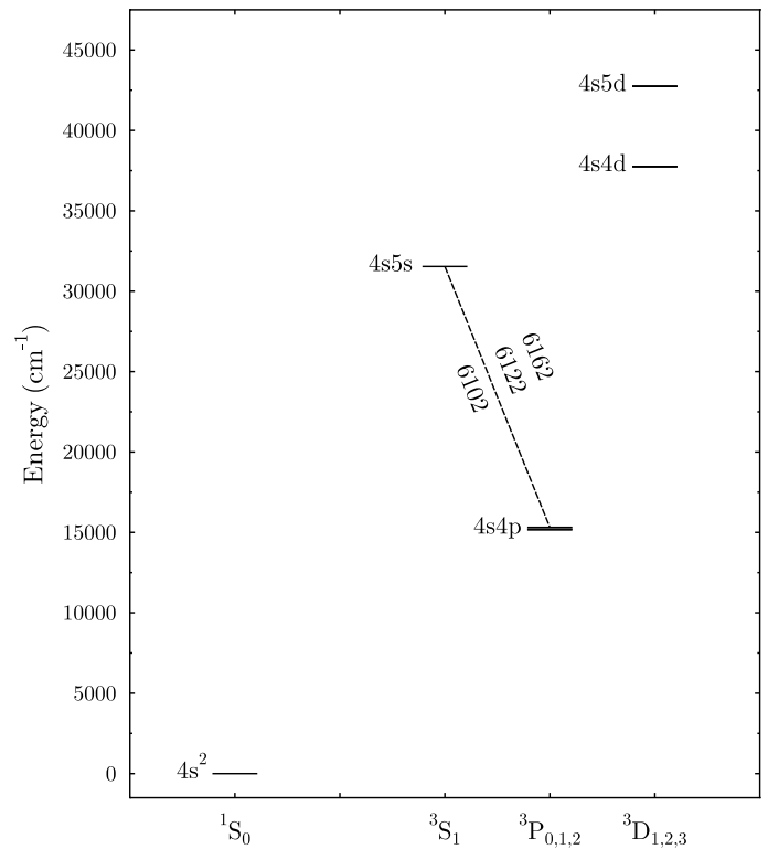
Fig. 2. Partial energy level diagram of Ca I displaying the ground state, the 4s4p\ ^3P levels and the levels for which the lifetimes were measured in the present work. The 4p–5s lines are marked with air wavelengths in Å.
