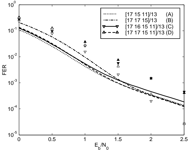
Figure 2: Bounds and simulations for Turbo codes with interleaver length 100 bits using the component codes in Table 1. Filled- and white faced markers correspond to Turbo codes with random- and correlation-designed interleavers respectively.
