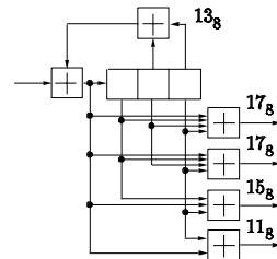
Figure 1: Low-rate component encoder with repeated use of generator polynomial 17_g .
