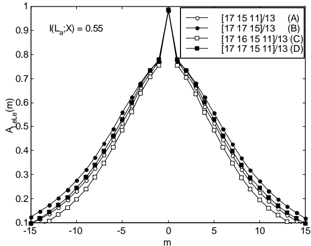
Figure 4: Correlation of extrinsic values after one APP decoding step for different component encoders. The extrinsic values are separated by m trellis steps, E_b/N_0 is equal to 1.0 dB and the mutual information I(L_a^{(k)}; X) equals 0.55.
