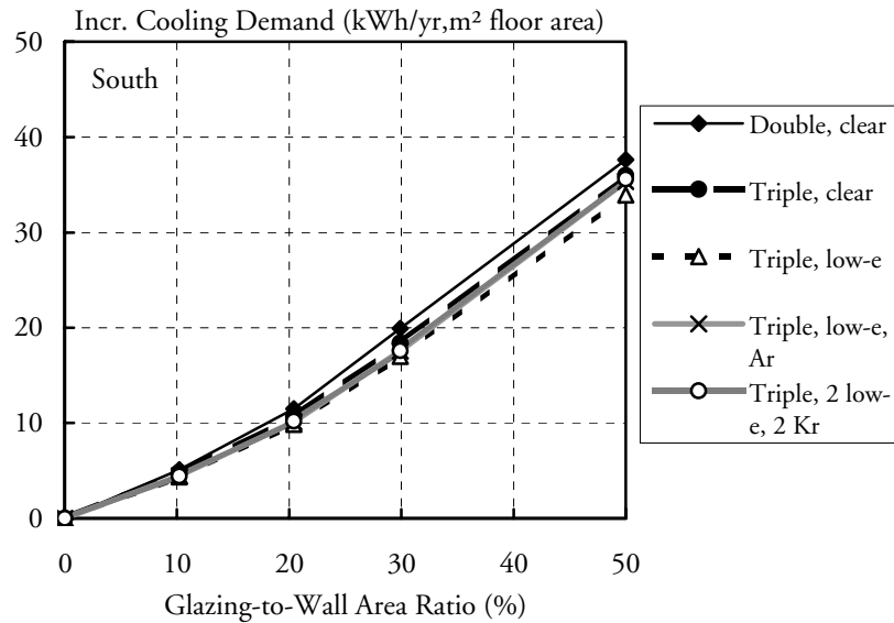
Figure 5.24 Incremental cooling demand ( \text{kWh/yr, m}^2 floor area) as a function of GVAR and window type for a south facing office in Lund
