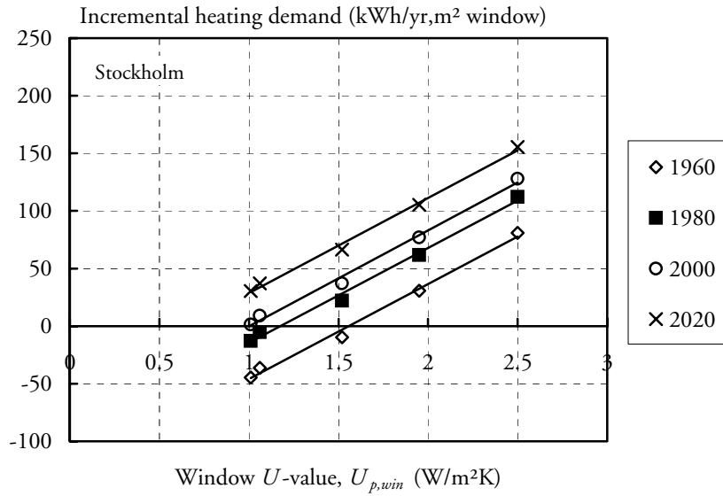
Figure 5.7 Incremental heating demand (kWh/yr, m² window area) as a function of window U-value and construction year of house. Simulations for Stockholm and window types 1-5 according to Table 5.2.
