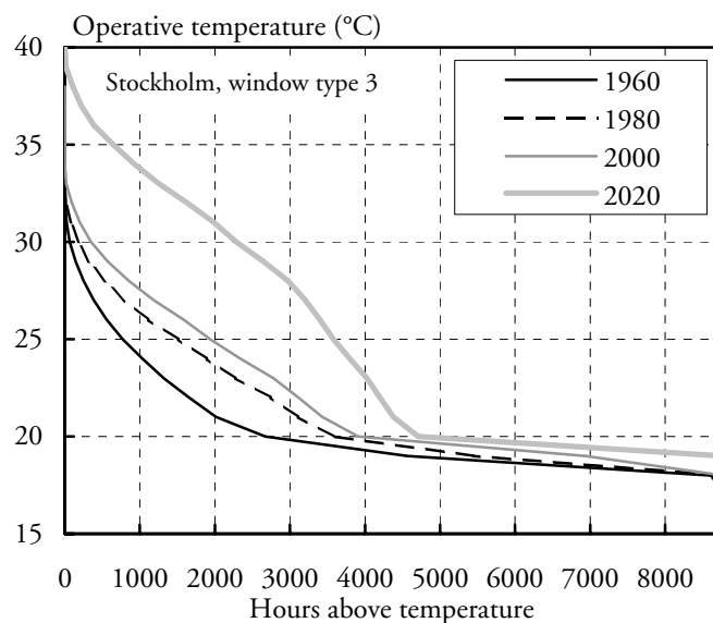
Figure 5.9 Global operative temperature ( ^{\circ}\text{C} ) of the ground floor (midpoint of room) as a function of construction year of house. Window type 3 in the Stockholm climate.
