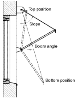
Figure 4 Section through window with awning, and definition of boom angle and slope.
