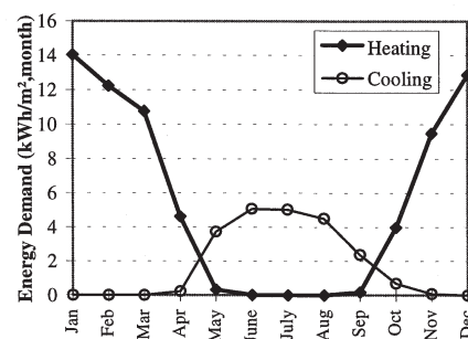
Fig. 3 The monthly heating and cooling demand (kWh/m 2 , month) of the base case.
