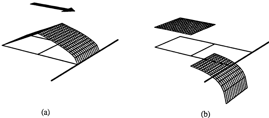
Fig. 4. The basis functions used to approximate the current perpendicular to an edge (a) and the corresponding charge distribution (b). The current basis function goes to zero as \sqrt{d} near the edge resulting in the singularity 1/\sqrt{d} for the charge.
