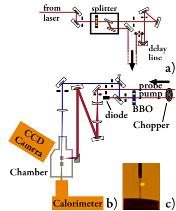
Figure 2.12. Optics setup for the table top XAS. a) The laser beam is split with a variable beam splitter. b) The repetition rate can be adjusted by a coupled chopper for pump and probe beam. The pump beam is converted into 400 nm, cleaned by two dichroic mirrors and focused into the chamber. The leakage from the first mirror is measured by a photodiode that will be fed into the detector to link pump and unpumped datapoints. The X-ray generating beam is reflected over a 90^\circ off axis parabolic mirror onto the water jet. c) The plasma is formed tangentially on a 160 \mu\text{m} water jet.
