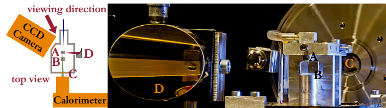
Figure 2.15. Magnified sample chamber and photograph of the setup. Debris protection and outer chamber walls have been removed. A is the water nozzle producing the water jet. B is an alignment pinhole in the place where the sample jet is placed. C is the entrance window of the Detector. D is the off axis parabolic mirror focusing the laser.
