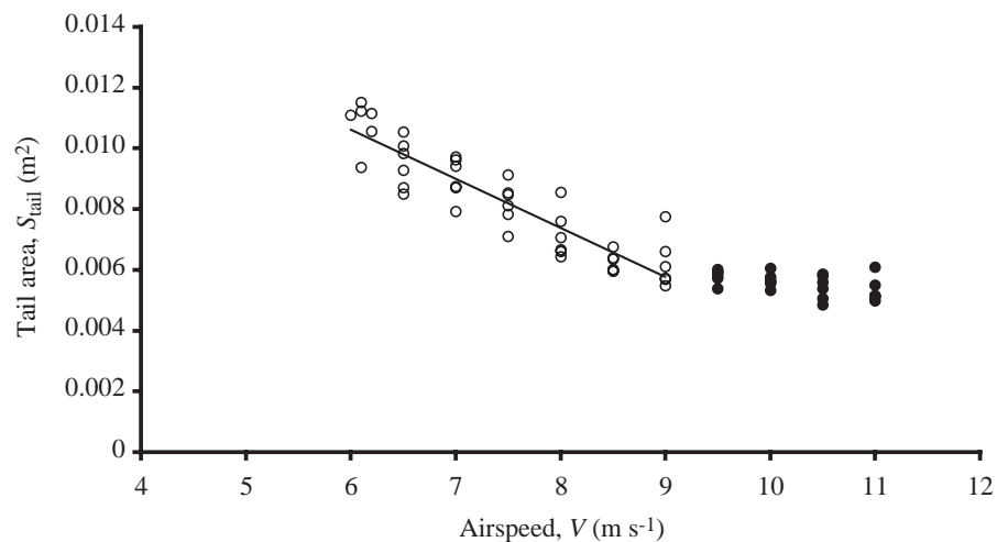
Fig. 5. Tail area S_{\text{tail}} with respect to airspeed V for a jackdaw in gliding flight. The tail area decreased linearly with speed between 6 and 9\text{ m s}^{-1} ( S_{\text{tail}}=-0.0016V+0.0203 , N=42 , r^2=0.83 , P<0.01 ). Above 9\text{ m s}^{-1} , the tail is completely folded and has the same area irrespective of speed ( S_{\text{tail}}=0.0056\pm 0.0004\text{ m}^2 , mean \pm s.d., N=24 ).
