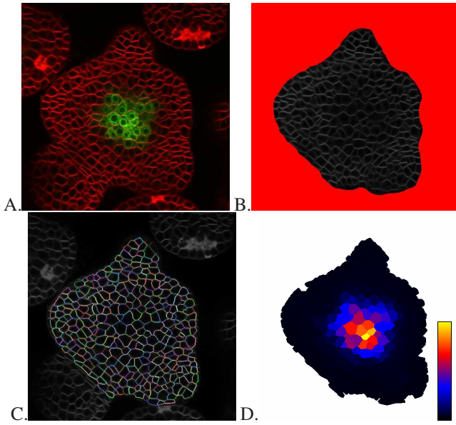
Fig. 3. Quantification of the WUS expression. A) A doubly labeled confocal image showing a horizontal section about 17 microns into the plant shoot. A cell membrane dye marker is shown in red, and fluorescence resulting from expression of a WUS::GFP construct is shown in green. B) Pixels extracted as background. As can be seen, older primordia are not included in the SAM template. C) Walls (defined by the borders between cell compartments) extracted by the watershed algorithm. D) Average GFP::WUS intensity for individual cells. These numbers are interpreted as relative concentrations. The color coding is defined by [black(min) - blue - red - yellow(max)].
