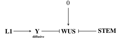
Fig. 5. A schematic illustration of the repressor model. The WUS expression is normally on ( 0 \rightarrow WUS ) in all cells. The WUS expression domain is restricted by the repressive signal described in Figure 4.
