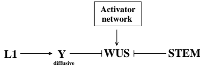
Fig. 4. A schematic illustration of the activator model. The activator network produce a pattern of an activator molecule which is inducing WUS. This activation is combined with a repressing signal originating from the surface layer of cells. The repressive contribution originating from the stem is not applicable in our two dimensional system, but is needed in a three dimensional model.
