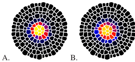
Fig. 8. WUSCHEL equilibrium concentrations in an unperturbed lattice simulation. A) Activator model. B) Repressor model. Color coding as in Figure 3.
