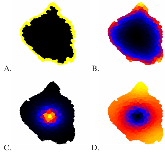
Fig. 7. Equilibrium concentrations for different molecules in the template simulation. A) L_1 is not updated and the figure shows the concentrations for both models. B) Y equilibrium concentration which is equal in both models. C) Equilibrium concentration of the activator A (only present in the activator model). D) Equilibrium concentration of B (only present in the activator model). Color coding as in Figure 3.
