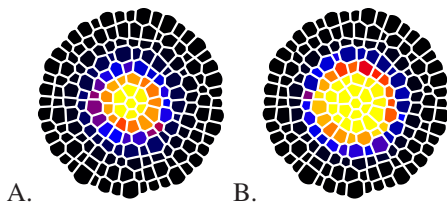
Fig. 9. WUSCHEL equilibrium concentrations in a simulation where the repressive signal is reduced by a factor two (The parameter V_y is set to half its original value for both models). A) Activator model. B) Repressor model. Color coding as in Figure 3.
