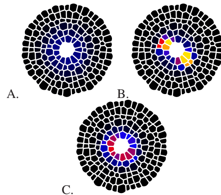
Fig. 10. WUS concentrations in the simulation of the laser ablation experiment. A) Early time point for the activator model. B) Equilibrium concentration for the activator model. C) Equilibrium concentration for the repressor model. Color coding as in Figure 3, where the maximal value is set to the maximal value in the unperturbed situation (Figure 8).
