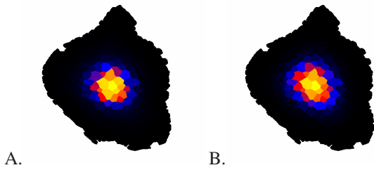
Fig. 6. WUSCHEL equilibrium concentration for both models simulated on the extracted template. A) Activator model. B) Repressor model. Color coding as in Figure 3.
