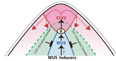
Fig. 1. A schematic figure of the expression domains of CLAVATA1, CLAVATA3 and WUSCHEL. The solid arrows indicate the regulatory (indirect) interactions, and the dashed arrows show the movement of the CLV3 protein.
