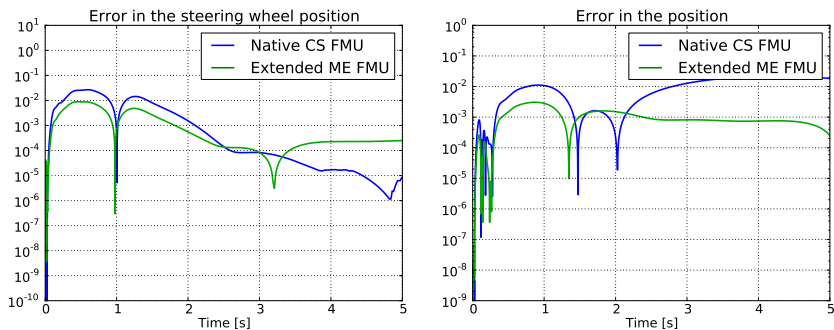
Figure 5.10: Comparison between a simulation of the monolithic model of the race car, in Section 5.4, as an model exchange FMU using the solver CVode from ASSIMULO with a relative tolerance of 10^{-8} with simulations of the coupled system, both using native FMUs and extended FMUs. The global step-size was H = 0.001 and iteration on the output variables was used. The left figure shows the difference of the position of the race car while the right figure shows the difference of the steering wheel angle.
