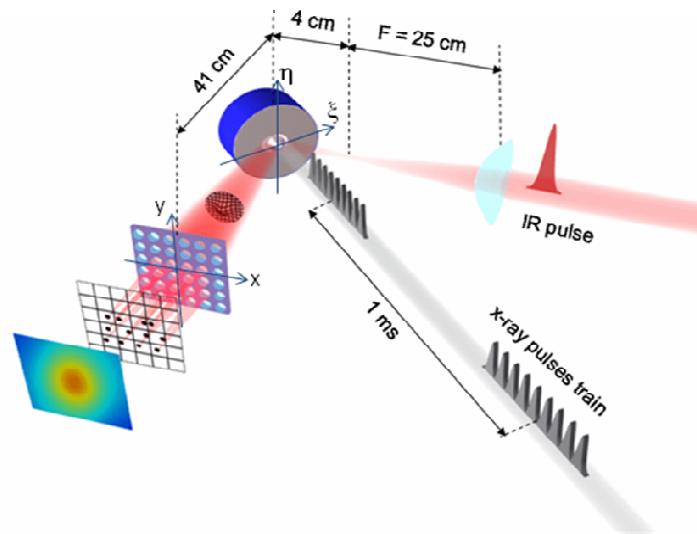
Fig. 1. Schematic view of the experimental setup
