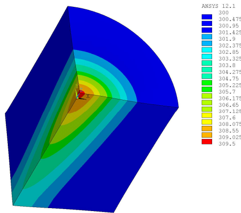
Fig. 5. Simulated volume with the FEM. The color shows the temperature in K at the end of the x-ray pulse train. The picture corresponds to the Si bare substrate.
