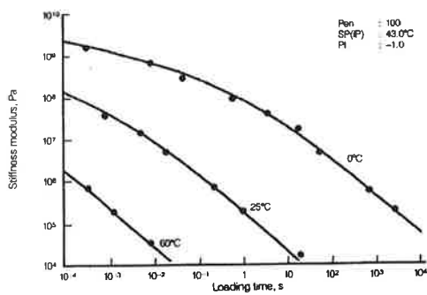
Effect of temperature and loading time on the stiffness of 100 pen bitumen
