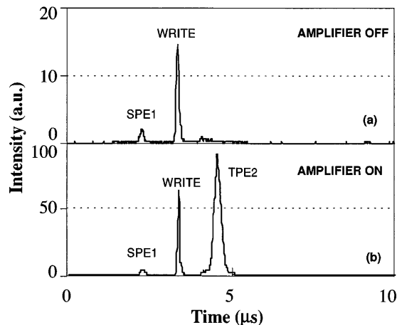
Fig. 2. Role of the amplifier in the generation of the REAP (TPE2) signal. Traces (a) and (b) are set to the same scale. The gain of the amplifier can be calculated to be \approx 180 .
