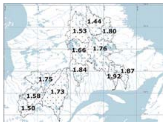
Figure 1: Long-term (1975-1999) observed mean annual runoff (mm/day).
