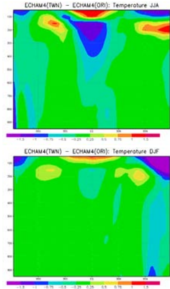
Fig. 3: 10 year seasonal zonal mean temperature difference [K] two-way-nested ECHAM4 – ECAHM4-only for boreal summer (upper panel) and boreal winter (lower panel).
