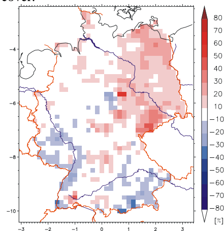
Fig 2. Relative difference between the 15-year mean annual precipitation simulated with MM5 and the corresponding reference data of DWD in percent.
