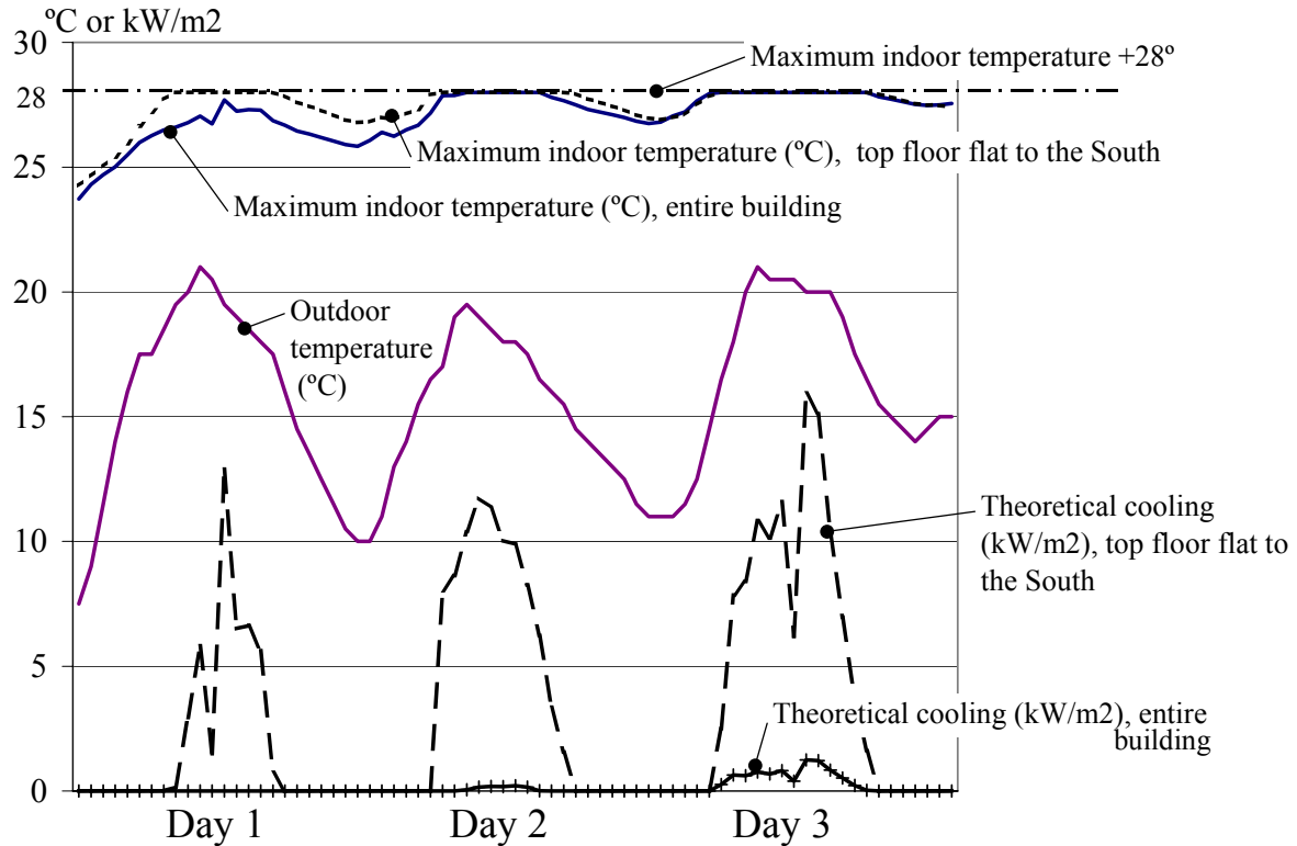
Diagram 5.1 Sequence of 3 consecutive days in June showing indoor temperatures and the cooling effect required to maintain a maximum indoor temperature of +28°C, for a specific solar exposed flat and the entire building. Calculation by VIP+(2000)
