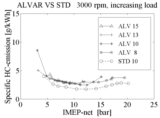
Figure 15. Specific HC - emissions. ( C_3H_8 equivalent).
