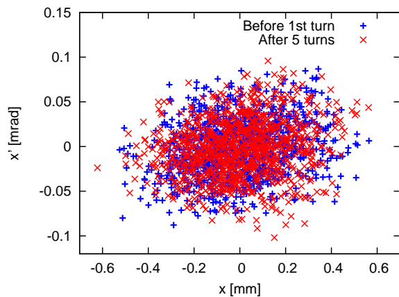
Figure 4: DIMAD tracking results at the 1.5 GeV IP showing the effect of the PSM in single-turn injection mode on the stored beam ( \varepsilon_x = 6 \text{ nm rad} , \sigma_\delta = 7.5 \times 10^{-4} , Gaussian distribution with cut-off at 3\sigma ).
