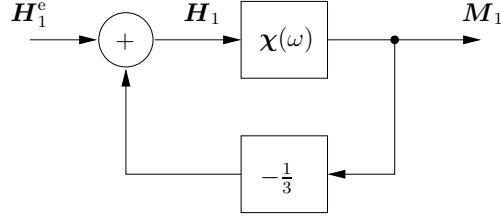
Figure 1: A system with negative feedback, corresponding to using a model where the external magnetic field is used as input. Even though the susceptibility \chi(\omega) is unstable with respect to its input \mathbf{H}_1 , the negative feedback makes the relation between the external field \mathbf{H}_1^e and the magnetization \mathbf{M}_1 stable.
