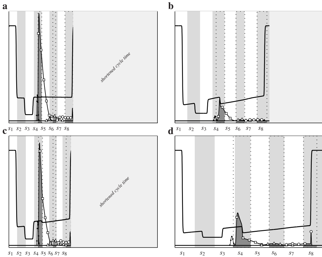
Figure 5: Simulations of the two-column MCSGP for the a) best productivity in Y-Pr b) best yield in Y-Pr c) best specific production in Y-Sp and d) best yield in Y-Sp for (-\bullet-) Nd; (-\square-) Sm; (-\triangle-) Eu; (-\circ-) Gd and the modifier (-) . The chromatogram is built up by joining s_1 to s_8 . The x axis is the volume eluted. Cut points for the pooling are seen as shaded peaks with dotted borders.
