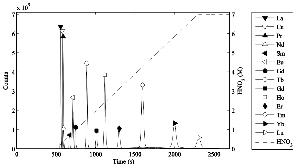
Figure 3: Chromatogram obtained with a ligand concentration of 345 mol/m 3 and a 30 min gradient. Both counts of the lanthanides and the nitric acid concentration, shown on the left and right y-axis respectively, correspond to the outlet of the column.
