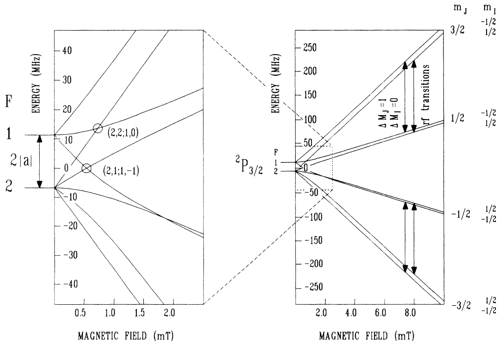
FIG. 2. Sublevel structure as a function of an external magnetic field for the ^2P_{3/2} state of ^{107}\text{Ag} . \Delta m = 2 level crossings are indicated using the symbols (F, m; F', m') designating the low-field quantum numbers for the participating sublevels. rf transitions in the Paschen-Back region of the hfs are also indicated.
