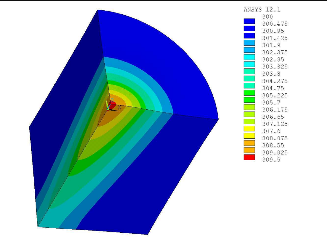
Figure 5: Simulated volume with the FEM. The color shows the temperature at the end of the x-ray pulse train. The picture corresponds to the Si bare substrate.
