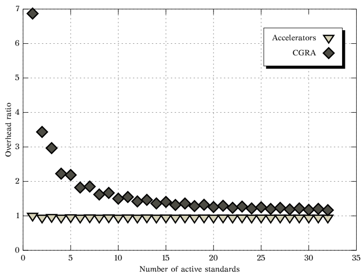
Figure 14.5.: Area Overhead of synchronization engine solution over accelerator solution shown for synchronization engine only, and full DFE-Rx.
