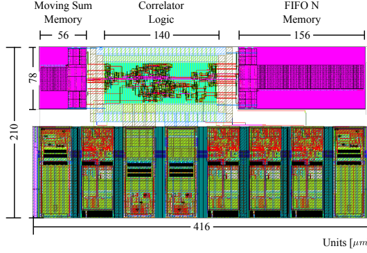
Figure 7.3.: Fabricated SB-time-freq-correlator in ST 65nm Technology with High VT low power cells.
