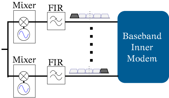
Figure 10.1.: Conceptual diagram of filtering based on a long FIR filter.
