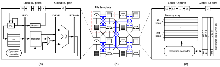
Figure 13.3.: (a) Building blocks in processor cell. (b) The CGRA is constructed from an array of processing and memory cells, connected using a local and a global hierarchical routing network. (c) Architectural block diagram of a memory cell.
