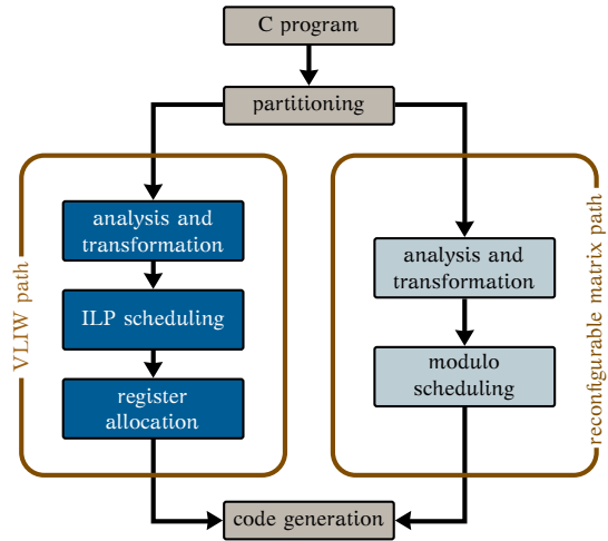
Figure 9.6.: ADRES compiler strategy.
