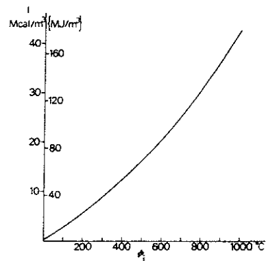
Fig. 11.1.5 c. Enthalpy I as a function of the insulation temperature \theta_i for slabs of mineral wool Type Minwool 3060 or Rockwool 337, of density \gamma_i = 150 \text{ kg/m}^3 . (According to the National Swedish Institute for Testing and Metrology)
