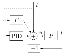
Fig. 9. Block diagram of the disturbance feed forward experiment.
