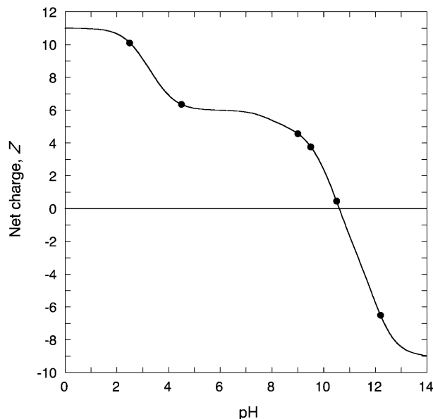
FIGURE 7 Net charge of monomeric BPTI as a function of pH, calculated from published \text{p}K_a values (Wüthrich and Wagner, 1979). The pH values of samples examined here are indicated by points.
