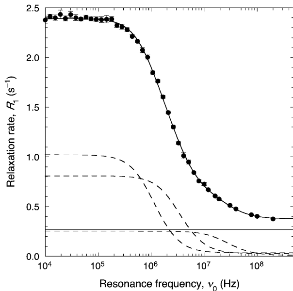
FIGURE 1 ^1\text{H} relaxation dispersion profile at 27 ^{\circ}\text{C} from an aqueous solution containing 14.5 mM BPTI and 0.90 M NaCl at pH 4.5. The dispersion curve resulted from a constrained 3-Lorentzian fit according to Eqs. 1–4. The individual Lorentzian components (dashed curves) and the bulk water contribution (horizontal line) are also shown.
