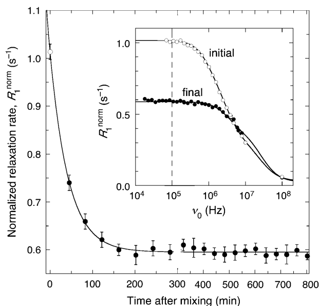
FIGURE 11 The insert shows ^1\text{H} relaxation dispersion profiles recorded at 27^\circ\text{C} from a 14.0\text{ mM} BPTI solution with 0.45\text{ M} NaCl and \text{pH } 4.5 , made by mixing equal volumes of two BPTI solutions with no salt and 0.90\text{ M} NaCl. The initial dispersion profile is the average of the (concentration normalized) profiles from the original solutions and thus corresponds to the initial nonequilibrium state obtained by suddenly reducing the NaCl concentration from 0.90 to 0.45\text{ M} . The final dispersion profile was recorded one week after the salt jump. The main figure shows the time evolution of R_1 , measured at 100\text{ kHz} (see dashed line in the insert ). Note the change of scale at 300\text{ min} on the time axis. The curve resulted from a three-parameter fit according to Eq. 6. Omission of the t = 0 point, taken from the initial dispersion profile in the insert, had no discernable effect on the fit.
