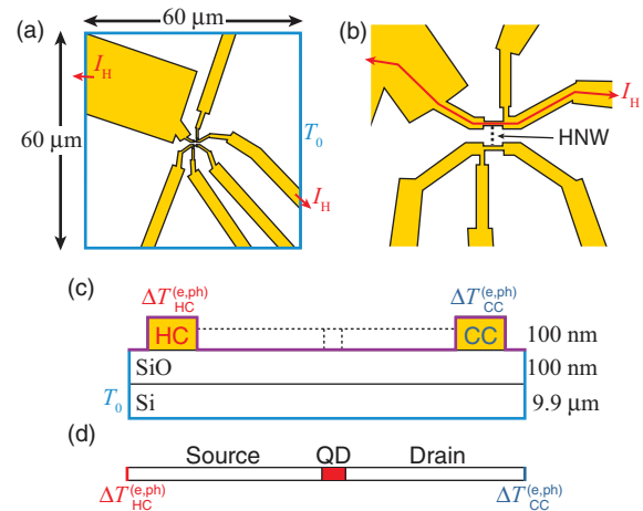
FIG. 3. (Color online) (a), (b) Top- and (c) side-view schematics of the simulated area for the Au leads and substrate, called the substrate simulations in the text. The location of where the HNWI would be is shown by dashed lines in panels (b) and (c). The outer boundary in (a) and lower boundaries in (c) (blue lines) are set to the background temperature T_0 . The top boundary in (c) (purple line) is assumed to be a perfect insulator. The red line in panel (b) shows the path of the heating current I_H . Panel (d) shows a schematic of the simulated HNWI. In panels (c) and (d), \Delta T_{HC}^{(e,ph)} and \Delta T_{CC}^{(e,ph)} represent the electron and phonon temperature rises in the HC and CC, respectively, as well as the boundary conditions for the simulated HNWI.
