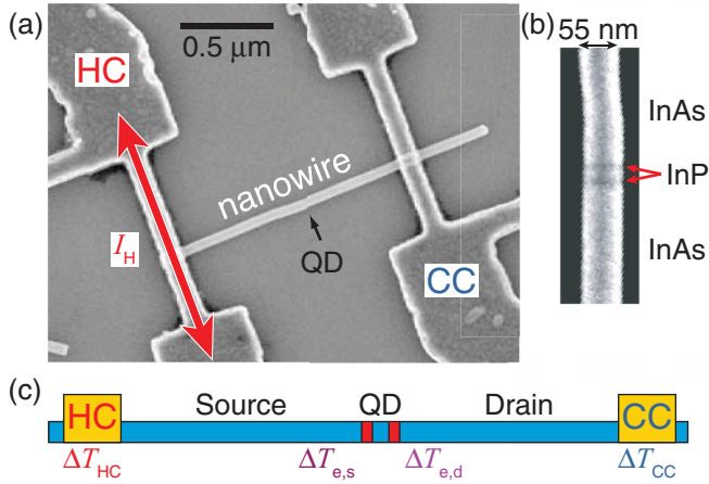
FIG. 1. (Color online) (a) A scanning electron micrograph (SEM) image of the HNW system showing the hot (HC) and cold (CC) Au contacts, and the approximate position of the quantum dot (QD), not visible here. A temperature gradient is applied using an ac heating current I_H through the HC. (b) Closeup SEM image of the two InP barriers within the InAs nanowire. (c) Cross section of the nanowire and contacts along the nanowire axis. \Delta T_{(HC,CC)} are the heating-induced electron temperature rises above the background temperature T_0 in the hot and cold contacts, respectively. \Delta T_{e,(s,d)} are the source and drain-electron temperature rises measured in the vicinity of the quantum dot. The source and drain portions of the NW are defined by the direction of heat flow, the source being closest to the HC.
