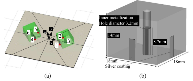
Fig. 5. (a) Simulation model of the compact DRA array. (b) Drawing of the single DRA prototype.
