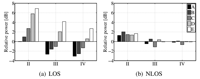
Fig. 10. Averaged RX power relative to Case I of each antenna system (Cases II - IV) at each measurement grid position (A - E).
