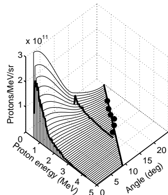
Figure 3.39. 3D interpolated surface illustrating the method for calculating the conversion efficiency. The spectra and divergence data are the same as in Fig. 3.38(a).
