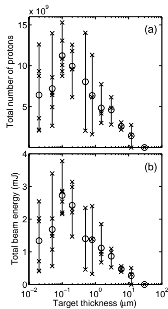
Figure 3.40. For protons above the detection threshold of the beam profile measurement (0.9 MeV): (a) Total integrated proton numbers. (b) Total integrated proton beam energy.
