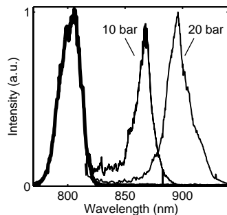
Figure 4.8. The reference laser spectrum (thick line) and two examples of Raman shifted laser spectra, corresponding to 10 and 20 bar backing pressure. Raman spectra have been cropped at 815 nm for clarity.
