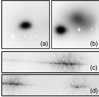
Figure 4.14. Electron beam profiles (a), (b) and corresponding Thomson scattered images of the channel, obtained for different intensity levels of the ASE pedestal. In (a) and (c), the contrast is 3 \times 10^7 . In (b) and (d) it is 2 \times 10^6 .
