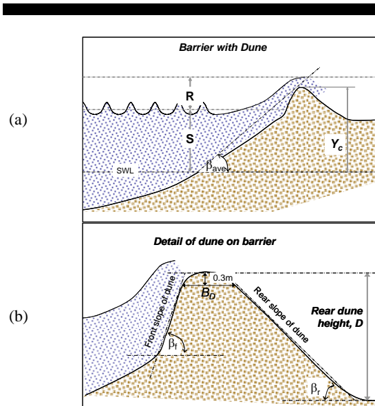
Figure 2. Schematic of (a) barrier (b) and detail of dune on barrier defining morphology parameters
