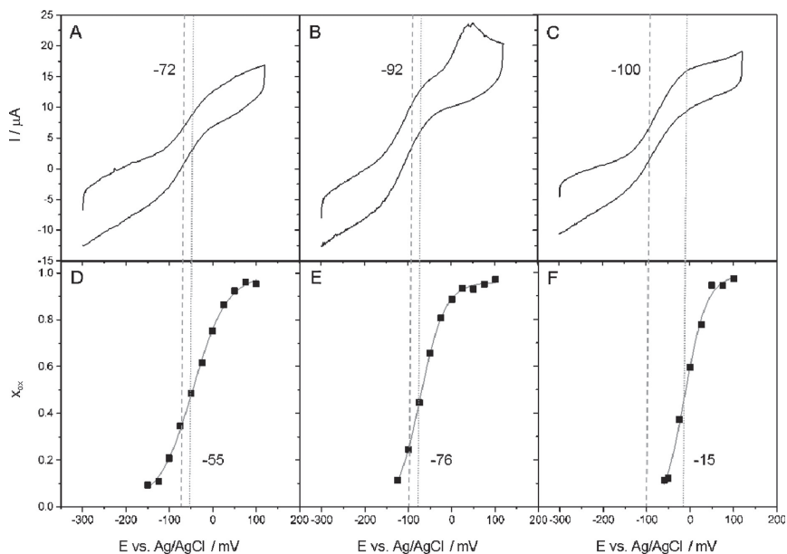
Figure 3. A)–C) Cyclic voltammograms of MtCDH under turnover conditions (10 mM of lactose, scan rate 100\text{ mVs}^{-1} ). Measurements were taken in A) 50 mM acetate buffer; B) 200 mM acetate buffer; C) 50 mM acetate buffer + 10 mM \text{CaCl}_2 buffer. Dashed lines (-----) refer to the inflection point of the curve. D)–F) Redox titration curves obtained from SERR measurements of immobilized MtCDH in the absence of lactose. The line represents a Nernst fit to the data. Measurements were taken in D) 50 mM acetate buffer; E) 200 mM acetate buffer; F) 50 mM acetate buffer + 10 mM \text{CaCl}_2 buffer. Dotted lines (.....) refer to the redox potential of the heme obtained from SERRs.
