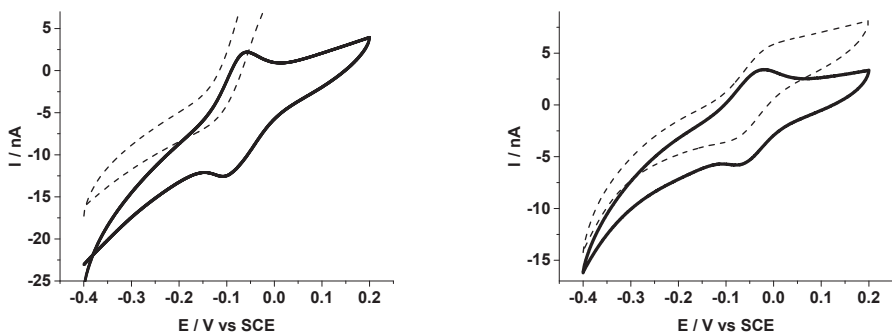
Figure 6. Cyclic voltammograms of class II CDHs (left) recCtCDH and (right) recMtCDH on MUOH modified gold electrodes at pH 3 at a scan rate of 5 mV/s in the absence (solid line) and in the presence of 1 mM lactose (dashed line)
