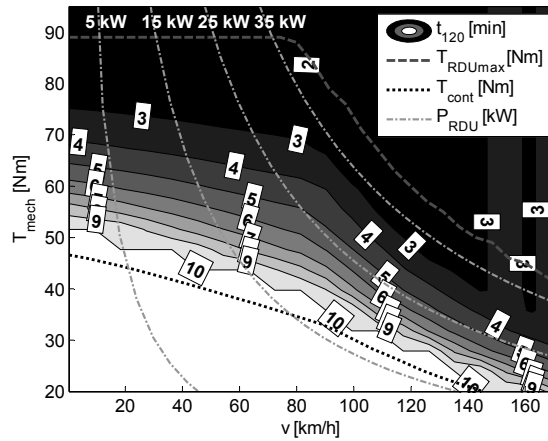
Figure 8.6 Time left, in minutes, before reaching the maximum temperature. The temperature of the cooling liquid is 25 °C, the initial temperature of the winding is 40 °C and the DC-voltage is 300 V.
