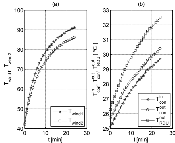
Figure 8.1 Winding temperatures (a) and cooling liquid temperatures (b) for the operating point, T_{\text{mech}} = 30 \text{ Nm} , f_c = 200 \text{ Hz}
