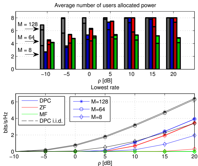
Fig. 7. Average number of users allocated power (top) and lowest ergodic rate (bottom) at site MS 2 when using 128, 64 and 8 antenna elements at the BS. Transmit power reduction has been applied.
