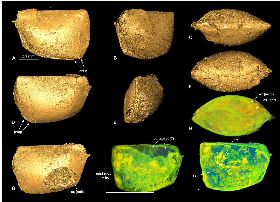
Fig. 3. A specimen of Heslondona ventrospinata (LO 12165t) with completely enclosed shield from the uppermost of Cambrian Series 3 ( Agnostus pisiformis Zone) at Transformatorstationen, Mount Kinnekulle, Västergötland, Sweden. A–G, 3D-rendering (isosurface) of a SRXTM dataset in different views; A, lateral view of left valve. B, antero-lateral view. C, dorsal view. D, lateral view of right valve. E, postero-lateral view. F, ventral view. G, lateral view with virtual cut through the shield and exhibiting parts of the mandibular exopod. H–J, 3D-rendering (semi-transparent images) of a SRXTM dataset in different views; H, ventral view. I, lateral view. J. lateral view, and specimen partly cut virtually. Abbreviations as in Figs. 1 and 2, additionally: pvsp, postero-ventral spine.
