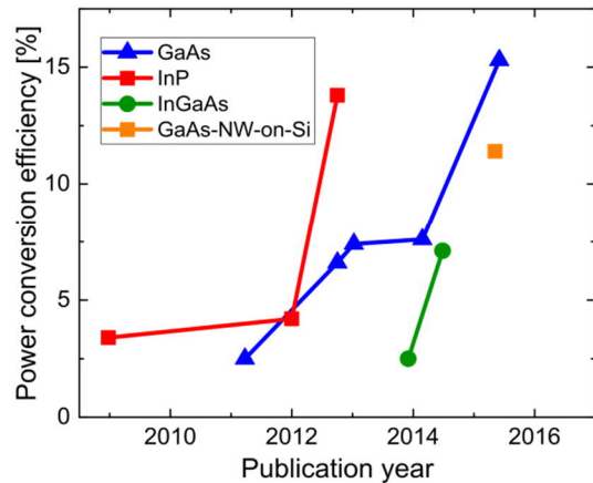
III-V nanowire array solar cell performance under one sun
