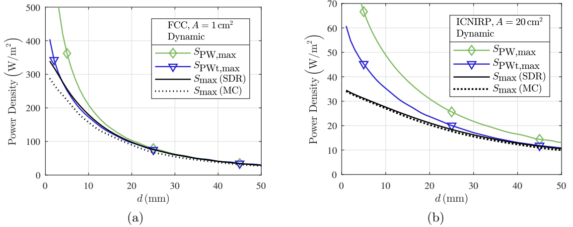
Figure 7: Comparison of S_{\max} produced by SDR and MC method, together with S_{\text{PW},\max} and S_{\text{PWt},\max} calculated by SDR, when |w_i|^2 \leq \zeta_{\text{ub}} , complying with (a) FCC limits, (b) ICNIRP limits.
