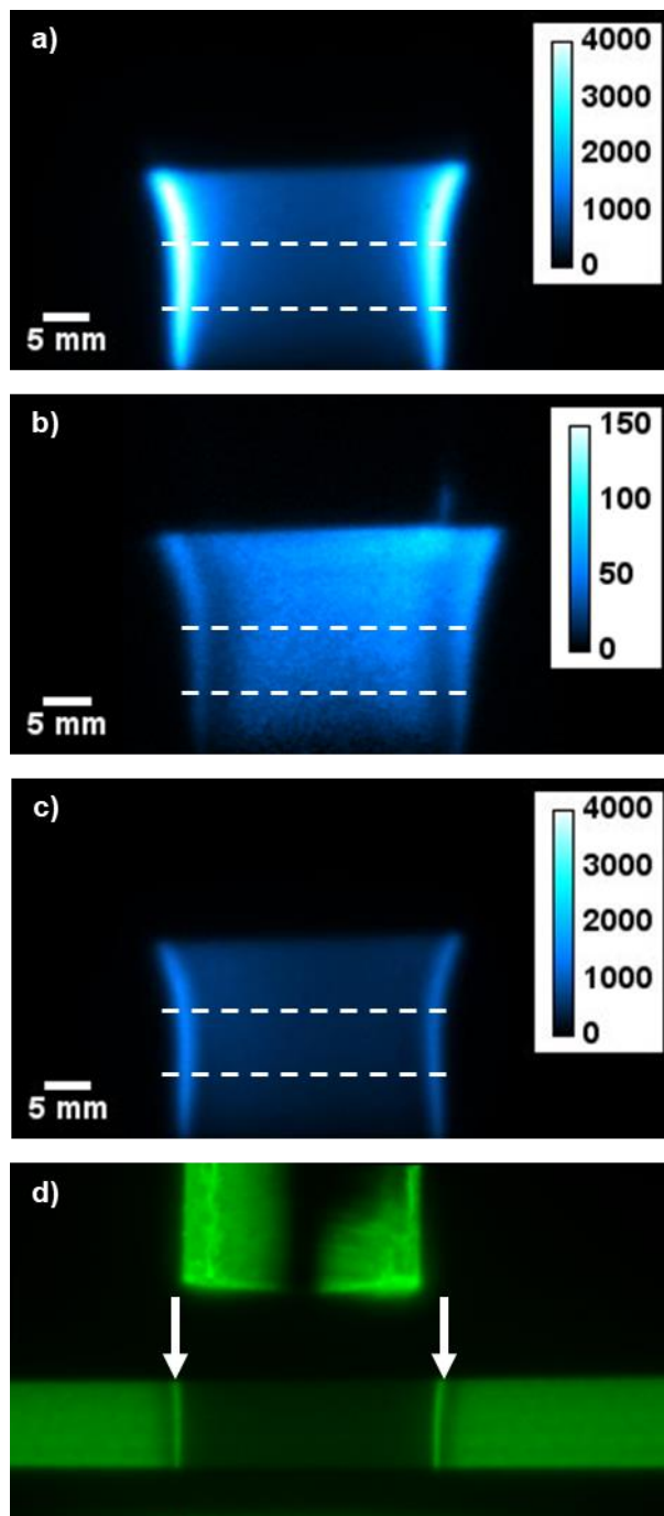
FIG. 3. Averaged (300 frames) photofragmentation fluorescence images measured in premixed methane-air flames of equivalence ratio \Phi=1.0 seeded with potassium compounds a) 0.5 M KCl b) 0.01 M KCl, and c) 0.5 M KOH d) Rayleigh scattering image measured in KCl-seeded (1.0 M) methane-air flame of \Phi=1.0 . Narrow regions of high signal at the flame edges, indicated by arrows, suggest KCl condensation. Temperature evaluation from Rayleigh scattering data was made for the regions between the horizontal lines in images a-c.
