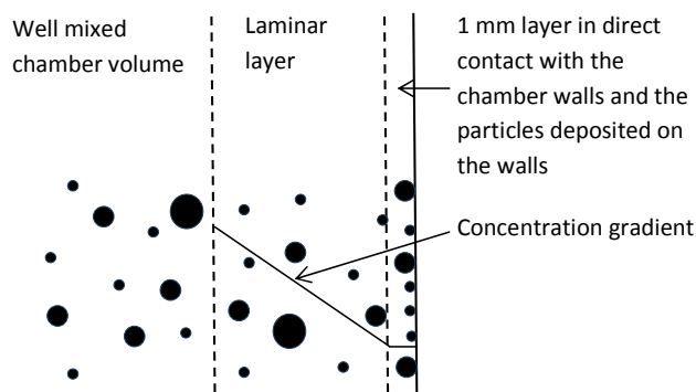
Figure 2. Schematic figure which illustrates how ADCHAM treats the diffusion-limited mass transfer of gas-phase compounds across a laminar layer next to the chamber walls. The thin (1 mm thick) air layer next to the chamber walls is treated as a separate volume which exchanges gas-phase compounds with the well-mixed chamber and the walls + wall-deposited particles.
