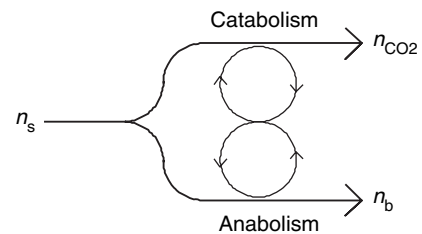
Figure 4 Schematic description of the division of aerobic metabolism into catabolism and anabolism. The molar quantities n_s , n_{CO_2} and n_b should be interpreted as moles of carbon (Cmol). The circles represent the ADP-ATP-cycle between the catabolic and the anabolic processes.
