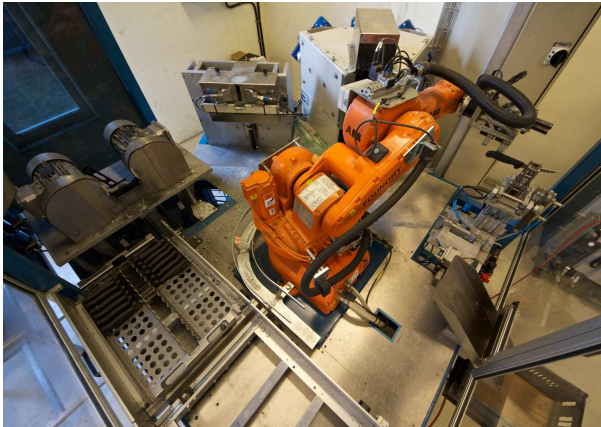
Fig. 3. The industrial knife grinding setup.
