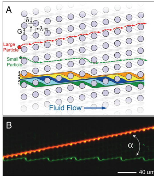
Figure 5.5. Deterministic lateral displacement. The asymmetrical placements of the posts in the array cause particles of different sizes to choose different flow streams. This results in an in lateral displacement and thus size separation. Printed with permission from Morton et al. [105]. Copyright 2008 National Academy of Sciences, U.S.A:
