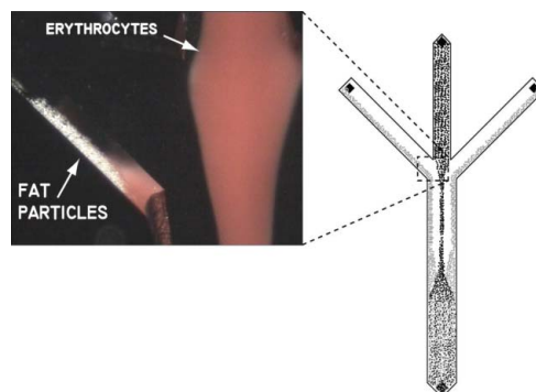
Fig. 11 Lipid particles separated from erythrocytes at the bifurcation of 350 \mu\text{m} separation chip with ultrasound turned on.
