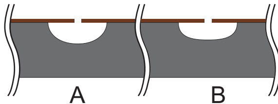
Figure 2.4. Isotropic etch profiles. A) is achieved by etching with agitation of the etch solution while B) is obtained without agitation.
