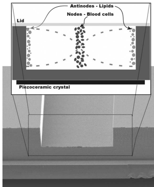
Fig 2. The principle of particle separation with ultrasound standing-wave technology. A scanning electron microscopy image shows the high-fidelity channels with vertical walls where separation is performed. Less-compressible particles with higher density (eg, erythrocytes) than the medium will move to the nodes, whereas more-compressible particles with a lower density (eg, lipid emboli) will gather at the antinodes.
