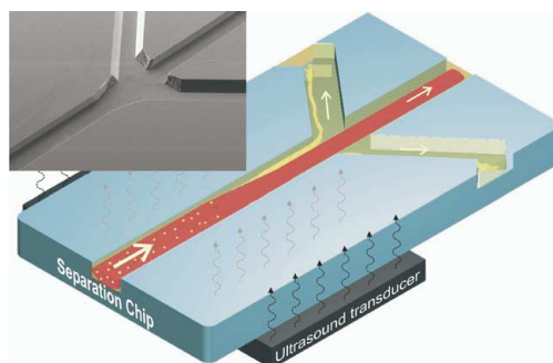
Fig 3. Schematic view of one 375- \mu m-wide separation channel and a scanning electron microscopic image of the trifurcation forming the center and side outlets in which the flow is divided depending on the acoustic properties of the particles. The orthogonal placement of the ultrasonic transducer is also depicted.
