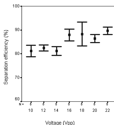
Fig. 10 Separation efficiency of a 45^\circ -structure as a function of the excitation voltage to the piezoceramic element. A constant frequency of 1.970 MHz, a flow of 0.3 \text{ ml min}^{-1} and 10% concentration of blood phantom was used.
