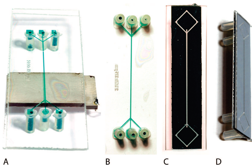
Figure 3. (A) Wet-etched glass chip with the piezoelectric element attached using ultrasonic gel. The back side of the glass chip with silicone tubing (B). The anisotropic silicon chip used for comparison can be seen in (C) and uses the same kind of silicone tubing for fluidic access from the back side (D).
