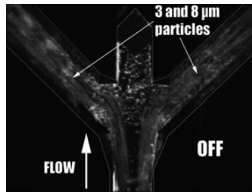
Figure 5.18a. Initial state with the ultrasound turned off. Both particle sizes exit through the side channels and the clear buffer through the middle. From Laurell et al. [27]
