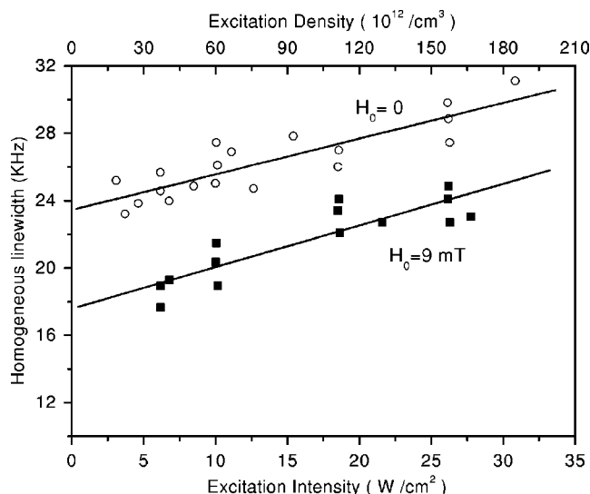
FIG. 2. Dependence of the homogeneous linewidths of the {}^1D_2 - {}^3H_4 transition on the density of excited ions in the presence and absence of an external magnetic field.
